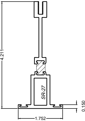
MULLION - FX/AWN & FX/CASEMENT SR-27
