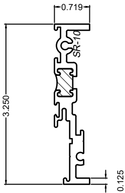
FRAME, NEUTRAL - FX/CASEMENT SR-10
