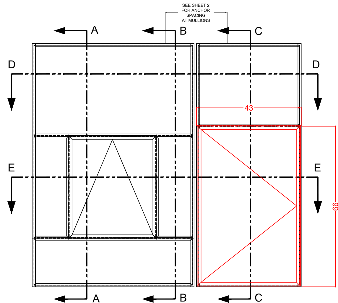
SEE SHEET 1 FOR SECTIONS & ANCHOR DETAILS AT PERIMETER AND KEY DIMENSIONS
