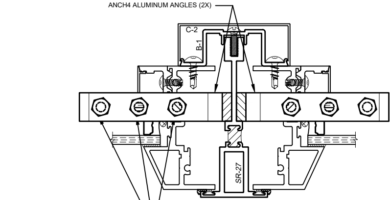
SECTION AT SILL
